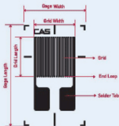
Strain Gauge Terminology
